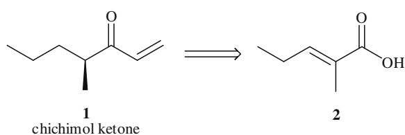
Scheme 1. Retrosynthetic analysis of chichimol ketone 1 .
